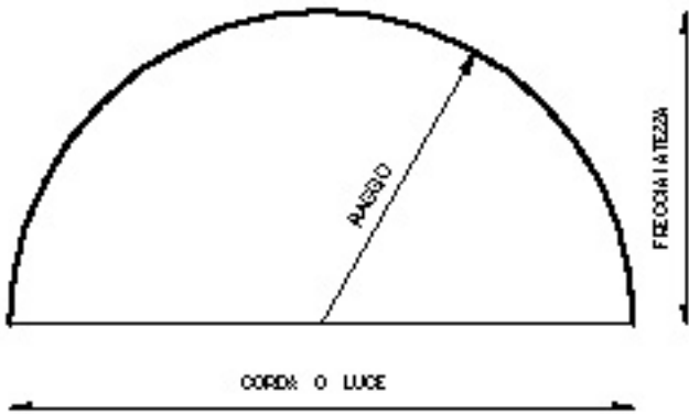
Roman arch or round arch
