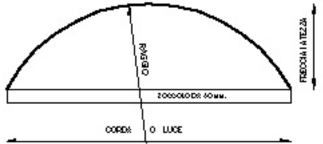
Depressed arch or longitudinal arch
